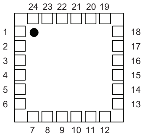
10mm x 10mm Land Grid Array (LGA) package
